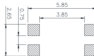
PCB. 焊接图 PCB. WELDING DRAWING
