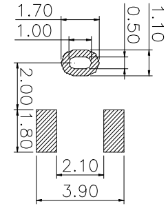
PCB. 焊接图 PCB. WELDING DRAWING
