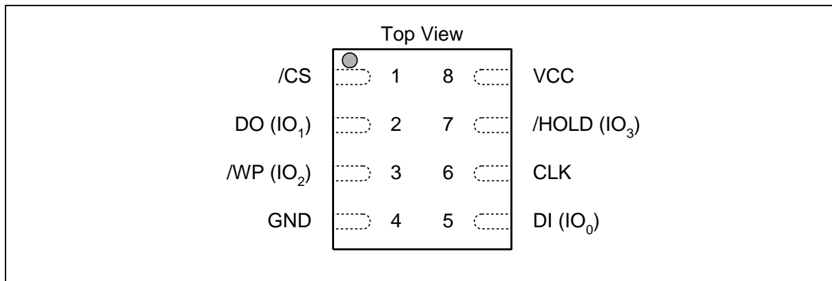
Figure 1b. W25Q40CL Pad Assignments, 8-pad USON 2x3-MM (Package Code UX)
