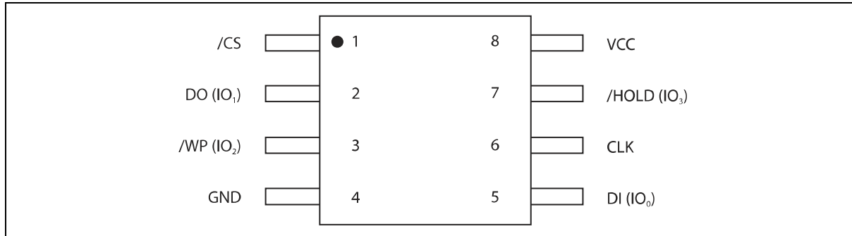
Figure 1a. W25Q40CL Pin Assignments, 8-pin SOIC 208-mi (Package Code SS)
