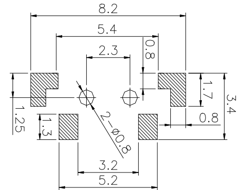
PCB. 焊接图 PCB. WELDING DRAWING
