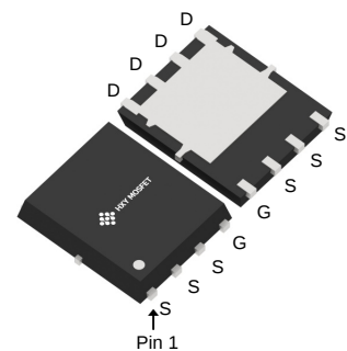
DFN5X6-8L (TDSO-8-EP(5x6))
