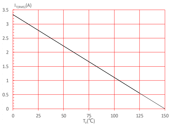
FIG.5: On-state characteristics
