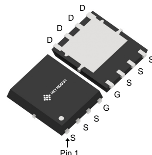
DFN5X6-8L
