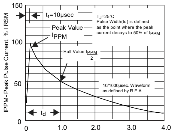
Fig.3 Pulse Waveform
