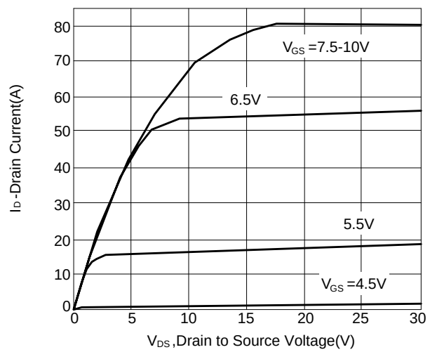
Figure 10: Output Characteristics
