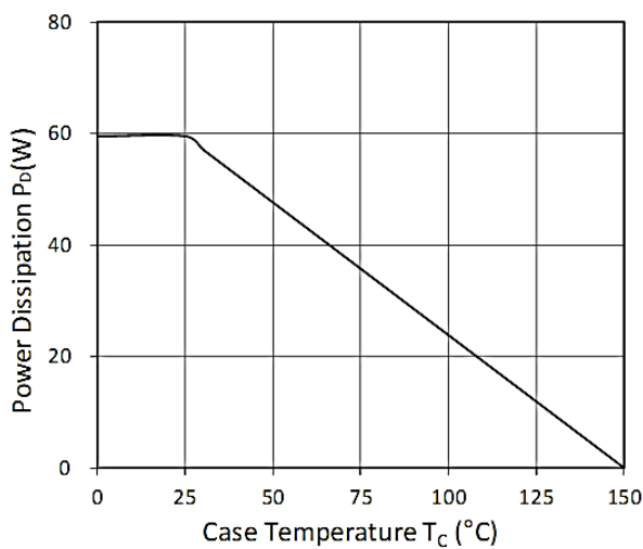
Figure 9. Power Dissipation
