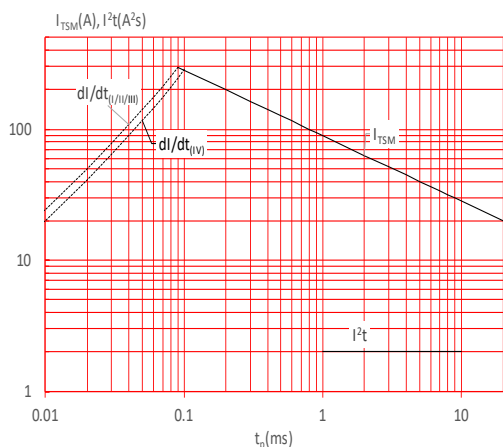
FIG.5: Non-repetitive surge peak on-state current for a sinusoidal pulse with width t_p < 20ms , and corresponding value of I^2t (I - II - III: di/dt < 50A/\mu s ; IV: di/dt < 30A/\mu s )
