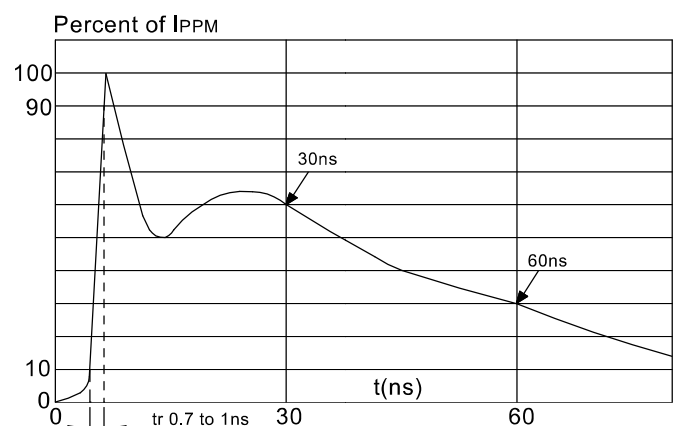
FIG.4: ESD clamping (8KV contact)
