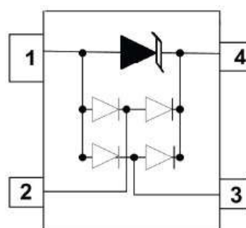
PIN Configuration
