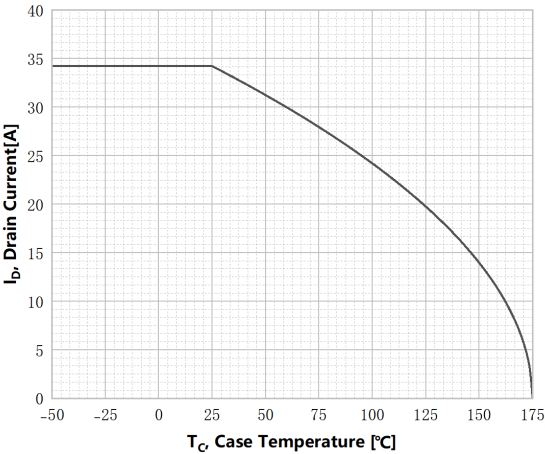
Figure 13. Continuous Drain Current Derating vs. Case Temperature
