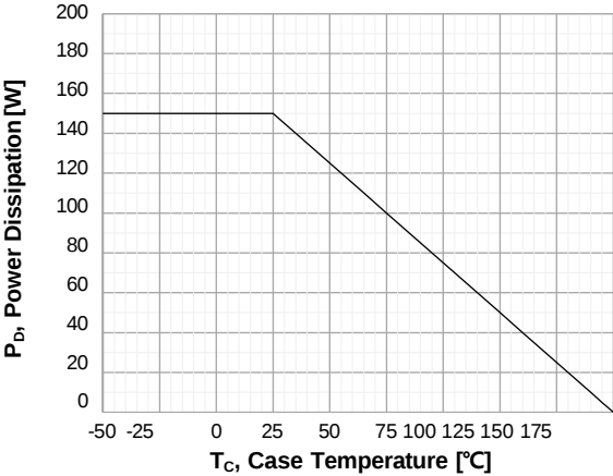
Figure 14. Maximum Power Dissipation Derating vs. Case Temperature
