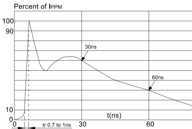
FIG.4: ESD clamping
