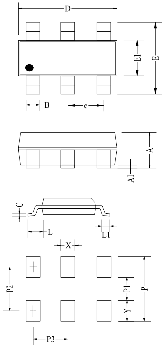
Land Pattern
