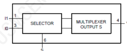
Figure 3. Logic diagram
