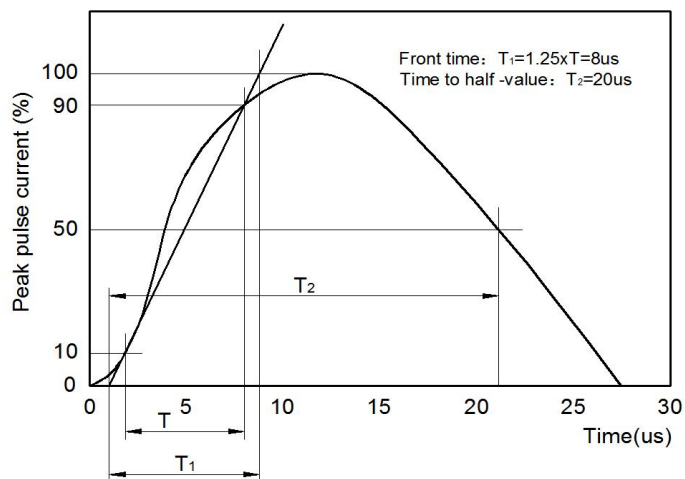
FIG3: Pulse Waveform
