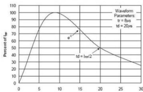
Pulse Waveform
