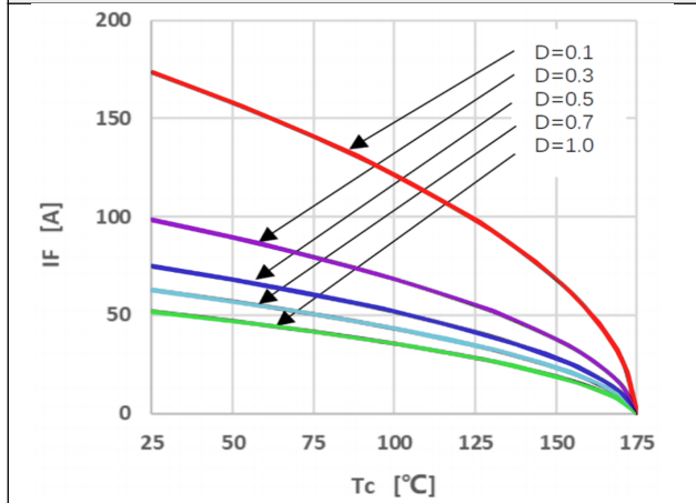
Figure 3. Peak Forward Current Derating
