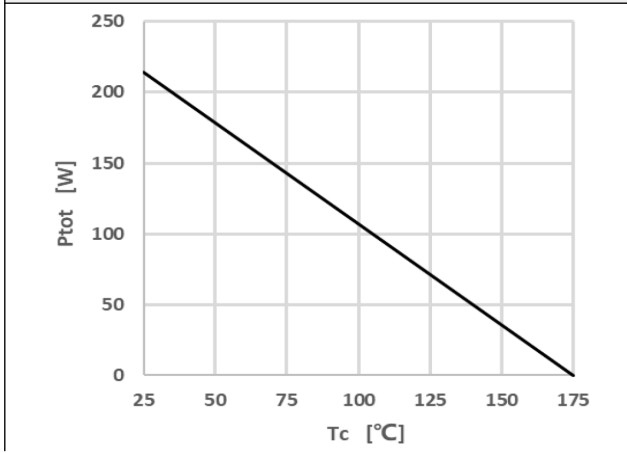
Figure 4. Power Dissipation
