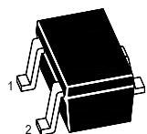
1.Base 2.Emitter 3.Collector SOT-323 Plastic Package
