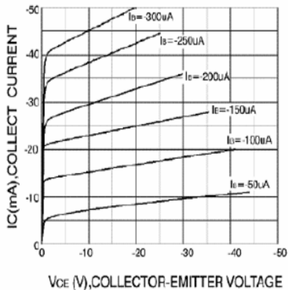
Static Characteristic
