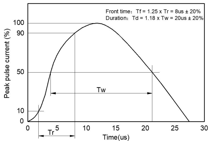
FIG2: pulse Waveform
