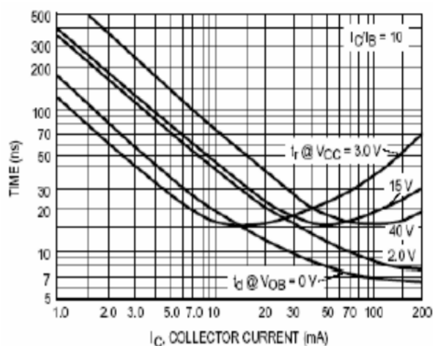
Figure 3 Turn-On Time
