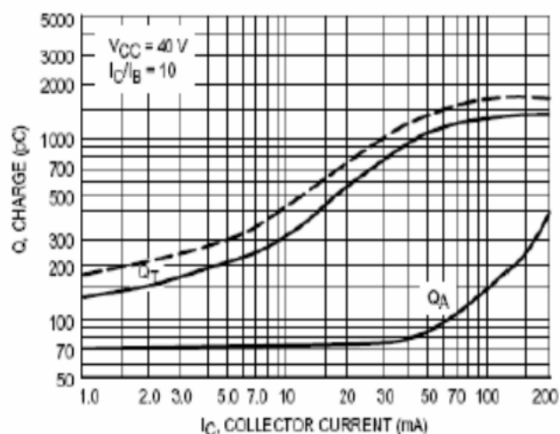
Figure 2 Charge Data
