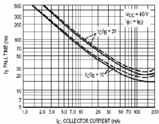
Figure 4 Fall Time
