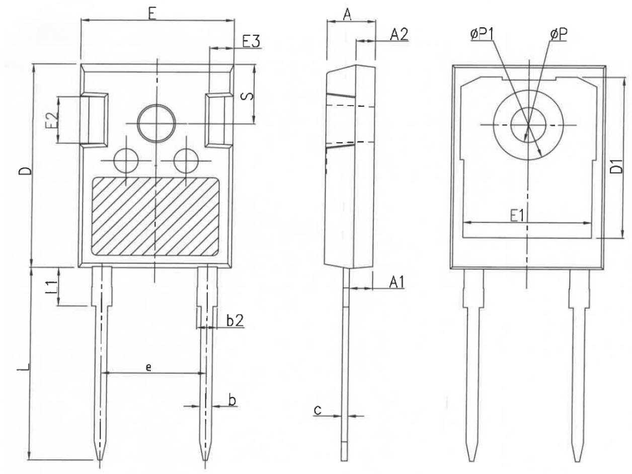
COMMON DIMENSIONS
