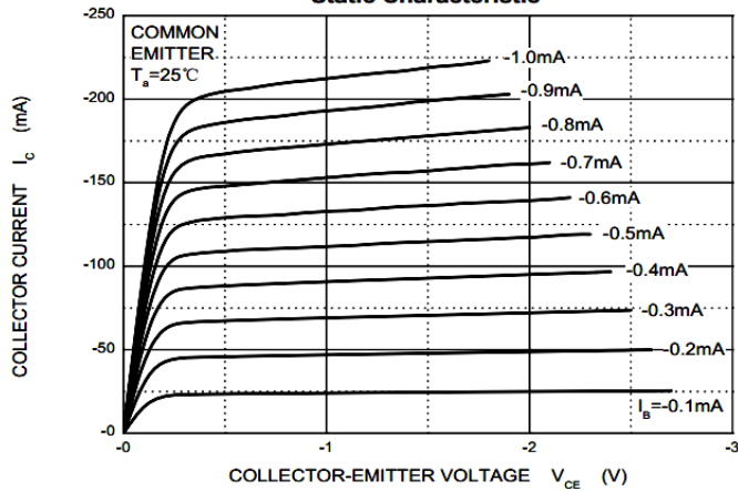
Static Characteristic
