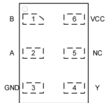
Fig 5. Top view pin configuration DFN6L
