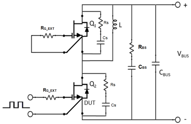
Figure 26. Schematic of the Half-bridge Mode Switching Test Circuit with Device RC Snubbers ( R_S = 10 \Omega , C_S = 100 pF) and a Bus RC Snubber ( R_{BS} = 2.5 \Omega , C_{BS} = 100 nF)
