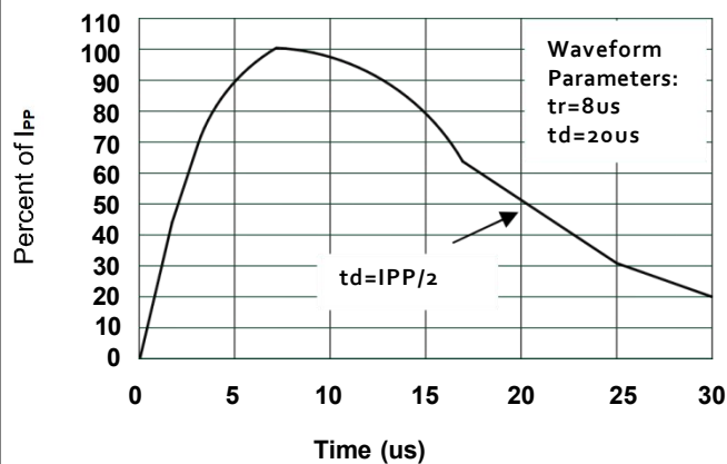
Pulse Waveform
