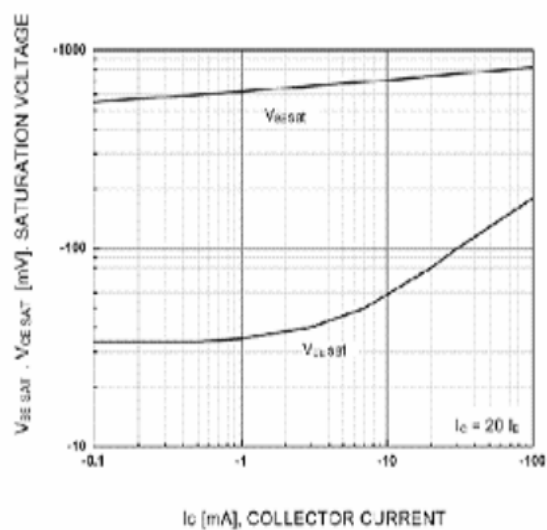
Figure 3. Base-Emitter Saturation Voltage Collector-Emmitter Saturation Voltage
