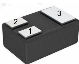
Package: DFN1006-3L 1: Base 2: Emitter 3: Collector
