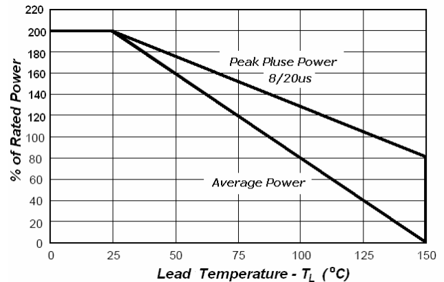
Fig2.Power Derating Curve
