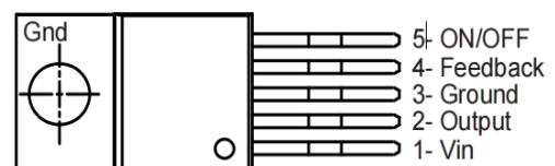
LM2575TB-XX
