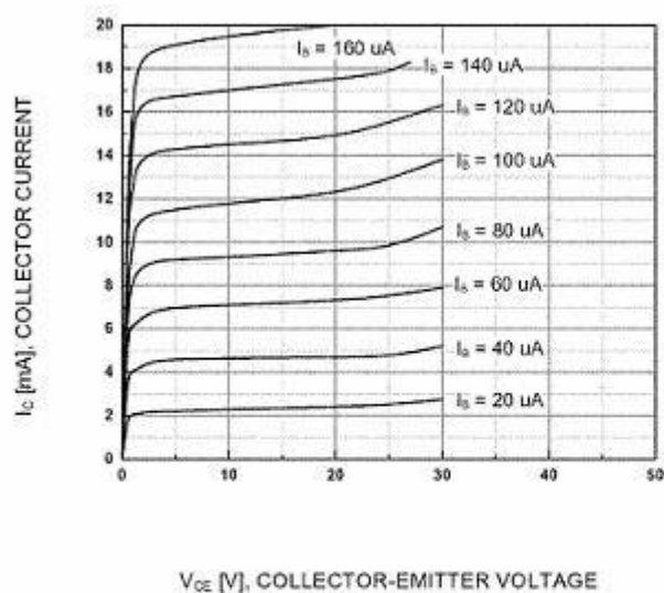
Static Characteristic
