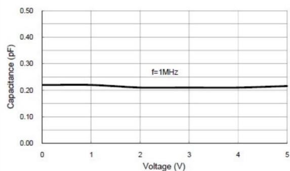
Fig 4 Voltage vs Capacitance I/O to I/O or GND
