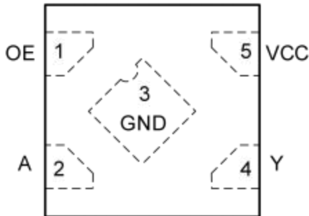
Fig 4. Top view pin configuration SOT23-5 and SOT353
