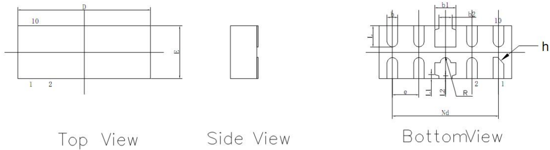
DFN2510 Package Outline
