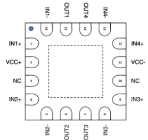
QFN-16 3*3
