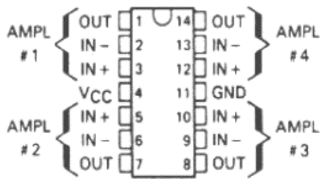
DIP-14/SOP-14/TSSOP-14
