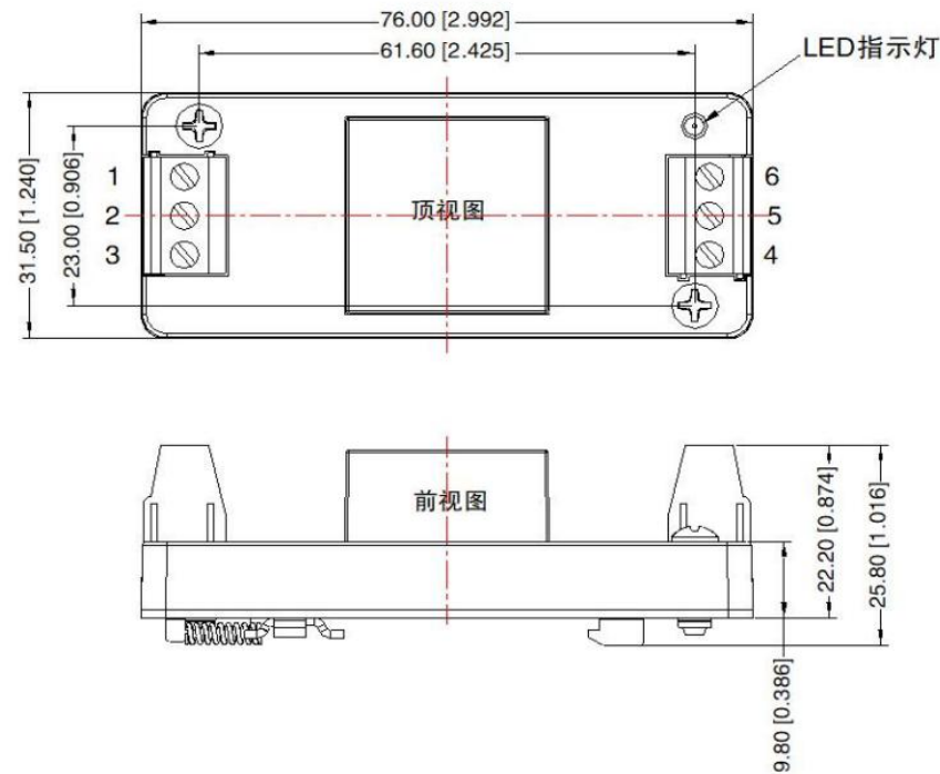
HVQ40-xxSxxV3CR 尺寸图
