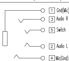
SCHEMATIC(PLUG OUT)
