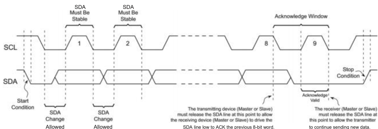
Figure 3-3.Start Condition, Data Transitions, Stop Condition and Acknowledge
