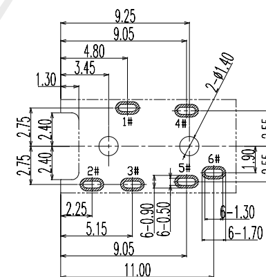
P.C.B LAYOUT T=1.00mm TOP VIEW
