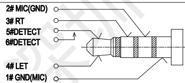
(Ø3.50mm 4 POLE PLUG SCHEMATIC )
