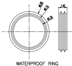
WATERPROOF RING
