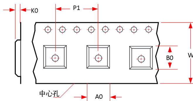
载带尺寸
