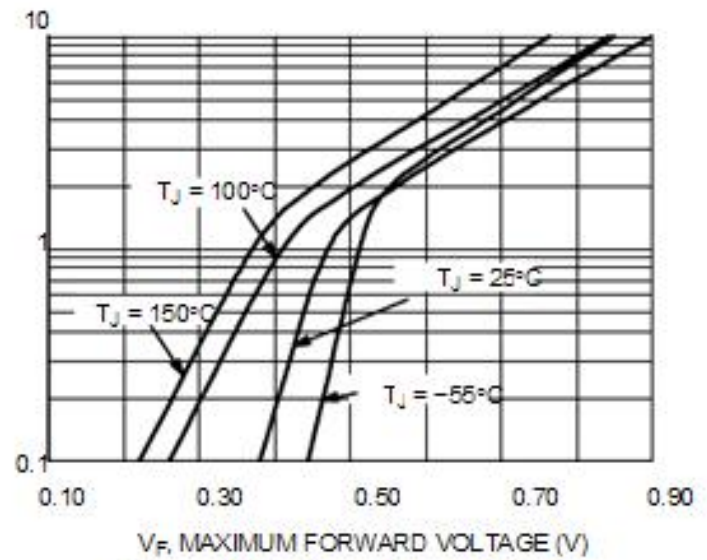
Figure 2. Maximum Forward Voltage
