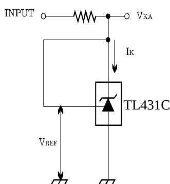
Fig.1. Test Circuit for V_{KA} = V_{REF}
