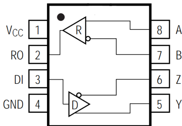
Figure 1. Pin Diagram
