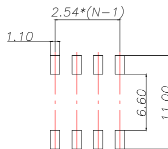
[P.C.B.LAYOUT]
