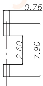
[P.C.B.LAYOUT]
