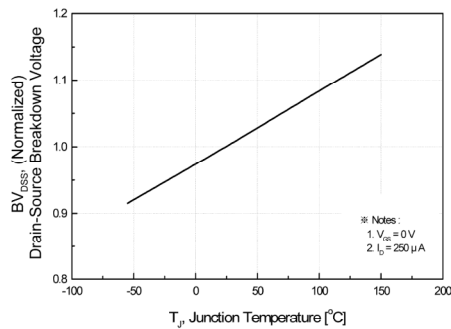
Fig 7. Breakdown Voltage Variation vs. Junction Temperature
