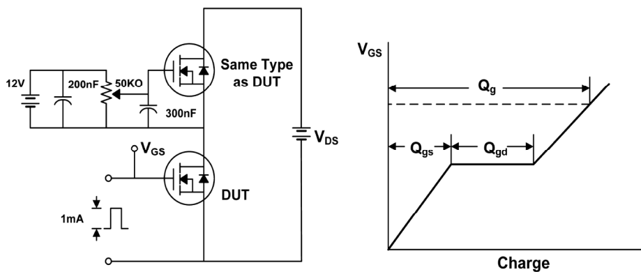
Fig 13. Switching Time Test Circuit & Waveforms
