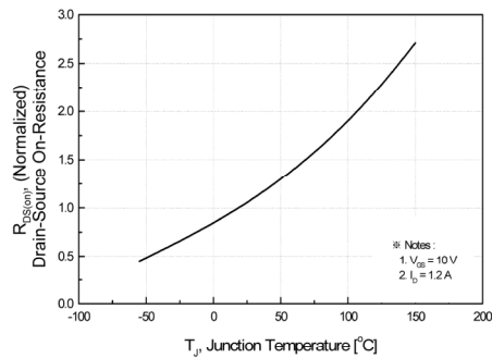
Fig 8. On-Resistance Variation vs. Junction Temperature
