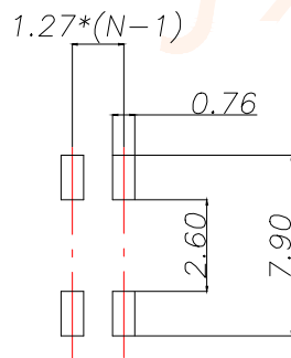
[P.C.B.LAYOUT]
