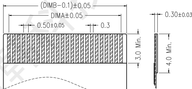
适用扁平线(Applicable Flat Cable)
